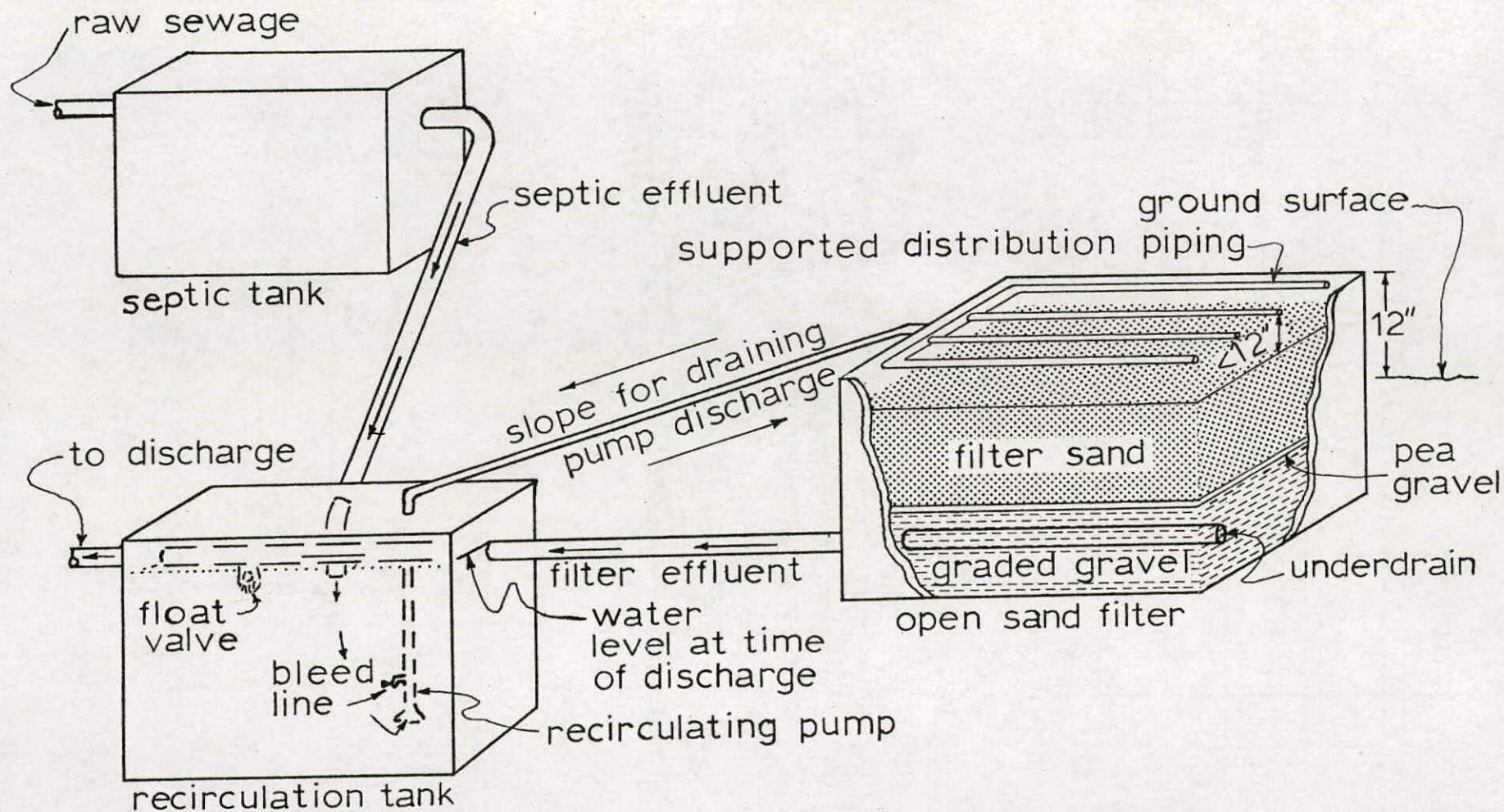
RECIRCULATING SAND FILTER SYSTEM
